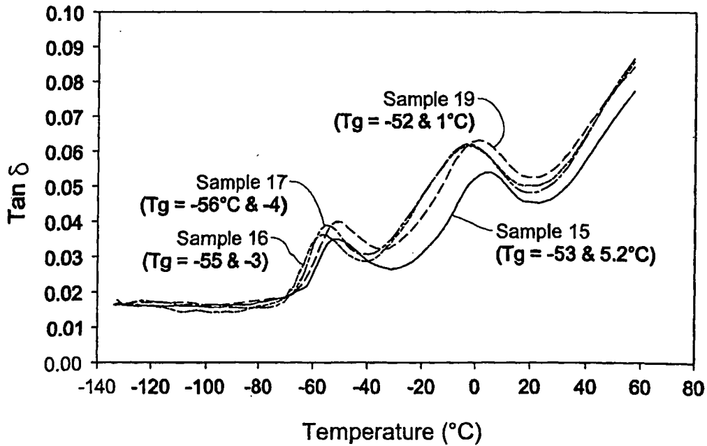
Fig. 4 Tan \delta of Plasticized Propylene Impact Copolymers
